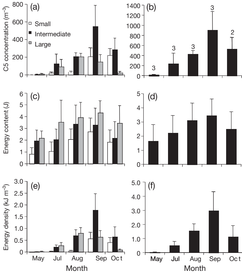
Fig. 9. Calanus finmarchicus . Histograms illustrating changes in monthly average (+2 SE) estimates in the Grand Manan Basin from May through October 2002 among (a,c,e) small, intermediate, and large size-classes of C. finmarchicus C5s and (b,d,f) all sizes combined; numbers over bar in (b): no. of collections analysed. (a,b) Concentration ( m^{-3} ), (c,d) individual gross energy content (J) and (e,f) gross energy density ( kJ m^{-3} )
