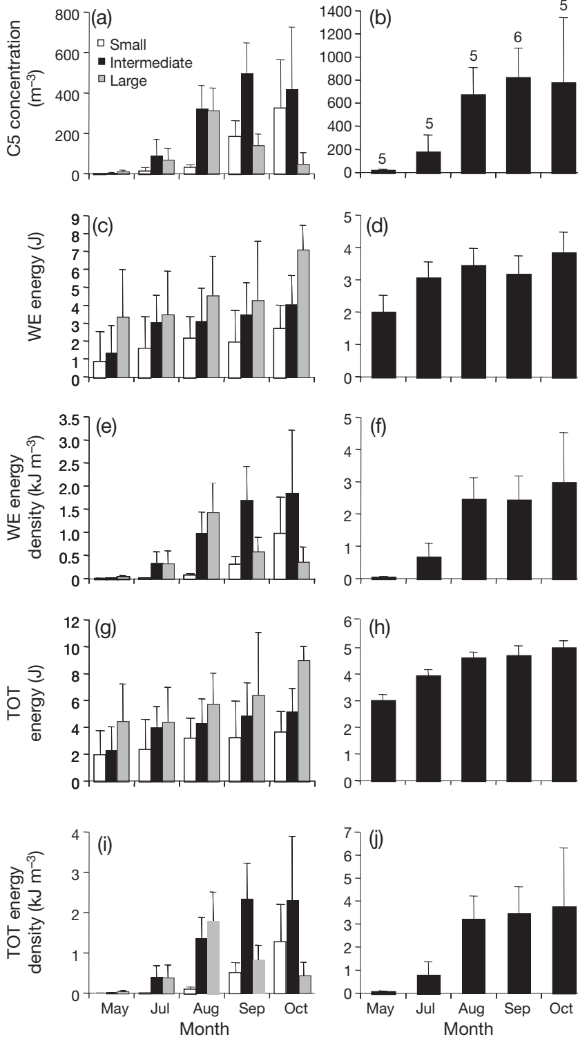
Fig. 10. Calanus finmarchicus . Histograms illustrating changes in monthly average (+2 SE) estimates in the Grand Manan Basin from May through October 2002 among (a,c,e) small, intermediate, and large C. finmarchicus C5 size-classes and (b,d,f) combined classes; numbers over bar in (b): no. of collections analysed. (a,b) Concentration ( \text{m}^{-3} ), (c,d) individual wax ester (WE) energy content (J), (e,f) WE energy density ( \text{kJ m}^{-3} ), (g,h) individual total lipid (TOT) energy content (J), and (i,j) TOT energy density ( \text{kJ m}^{-3} )
