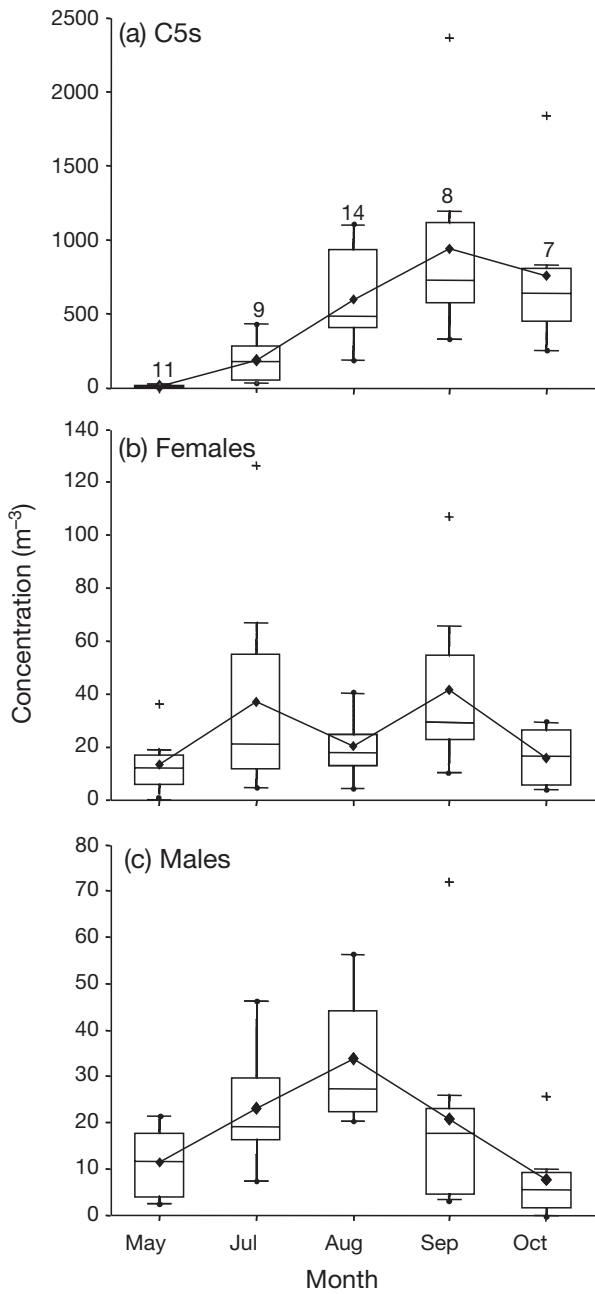
Fig. 4. Calanus finmarchicus . Box and whisker summary of depth-integrated estimates of (a) C5, (b) female, and (c) male C. finmarchicus concentration ( m^{-3} ) in the Grand Manan Basin from May through October 2002. The box and line represent the lower quartile, median, and upper quartile, the diamonds represent the mean, and the whiskers represent 1.5\times the inter-quartile range with outliers represented by crosses, absence of outliers by dots on the whisker. Numbers over box: no. of collections for each month
