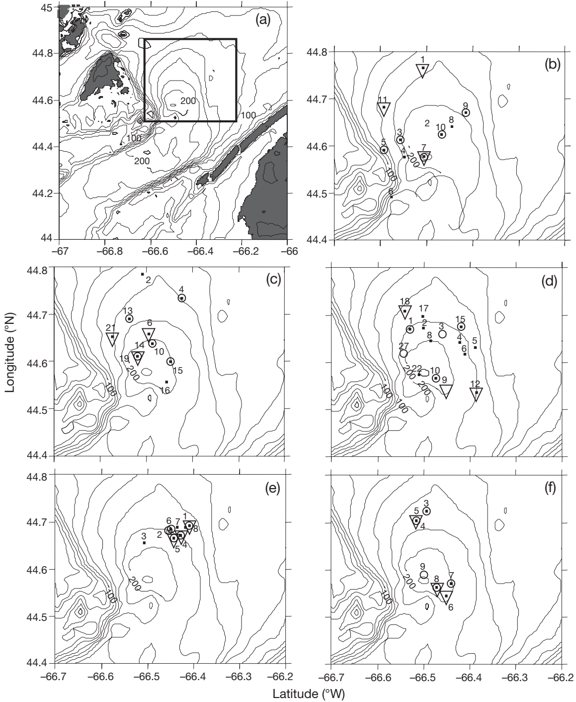
Fig. 1. Bathymetric (20 m resolution) charts of Grand Manan Basin, Bay of Fundy showing (a) the right whale conservation area (black box) and zooplankton collection stations occupied in (b) May, (c) July, (d) August, (e) September, and (f) October 2002 and those used to estimate zooplankton concentration (squares), copepod lipid content (circles), copepod total energy content (triangles). Numbers on charts indicate station identifiers
