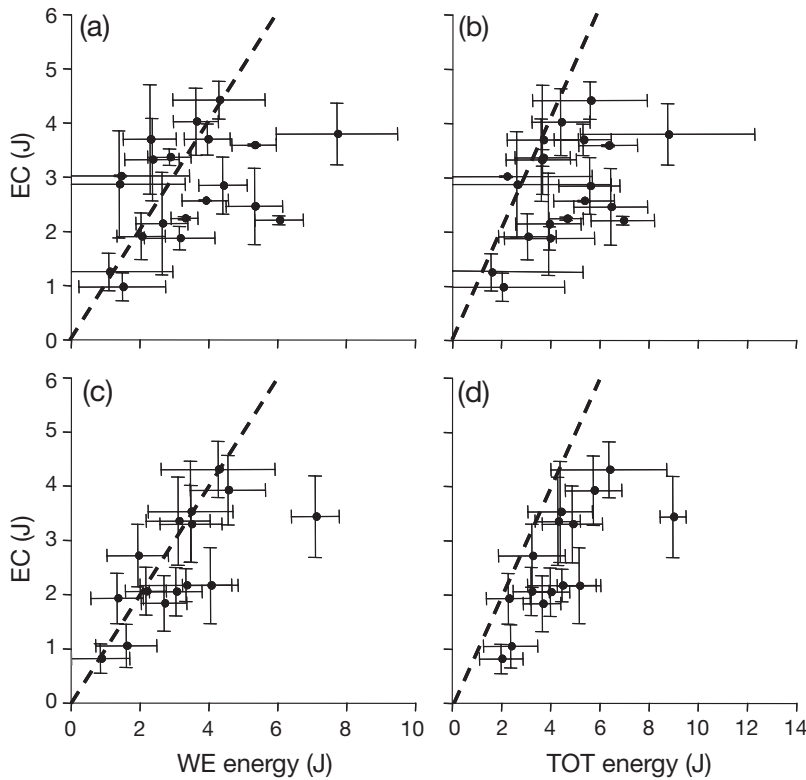
Fig. 11. Calanus finmarchicus . Relations between individual C5 total energy-content (EC; J) and wax ester (WE) and total lipid energy-content (TOT, J) based on (a,b) C5 size-class and collection basis and (c,d) C5 size-class and monthly average. Dashed line illustrates a 1:1 relation
