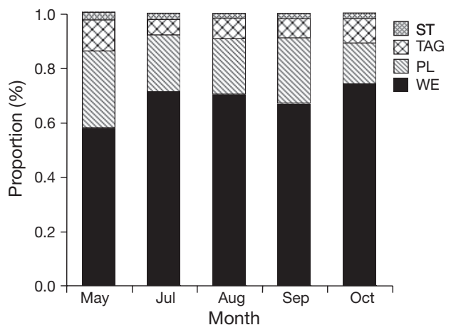
Fig. 7. Calanus finmarchicus . Monthly change in proportions of lipid components: wax esters (WE), polar lipids (PL), triacylglycerols (TAG), sterols (ST) in C. finmarchicus C5s in the Grand Manan Basin from May through October 2002
