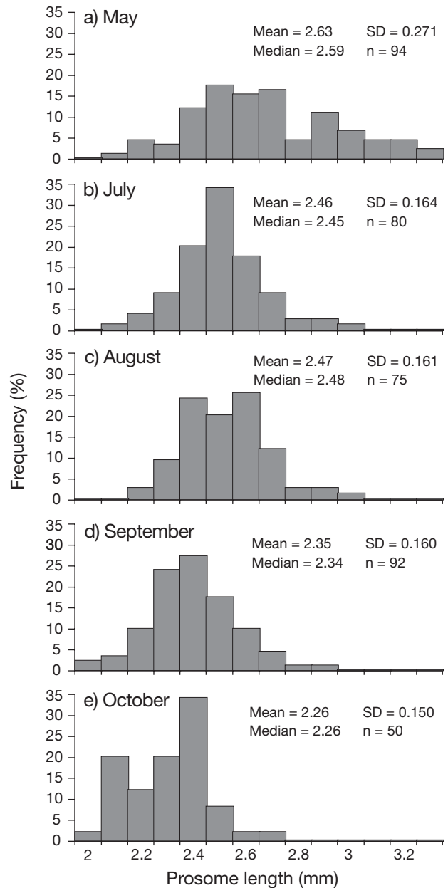
Fig. 5. Calanus finmarchicus . C5 prosome length (mm) frequency distributions and associated statistics for collections in the Grand Manan Basin during (a) May, (b) July, (c) August, (d) September, and (e) October 2002
