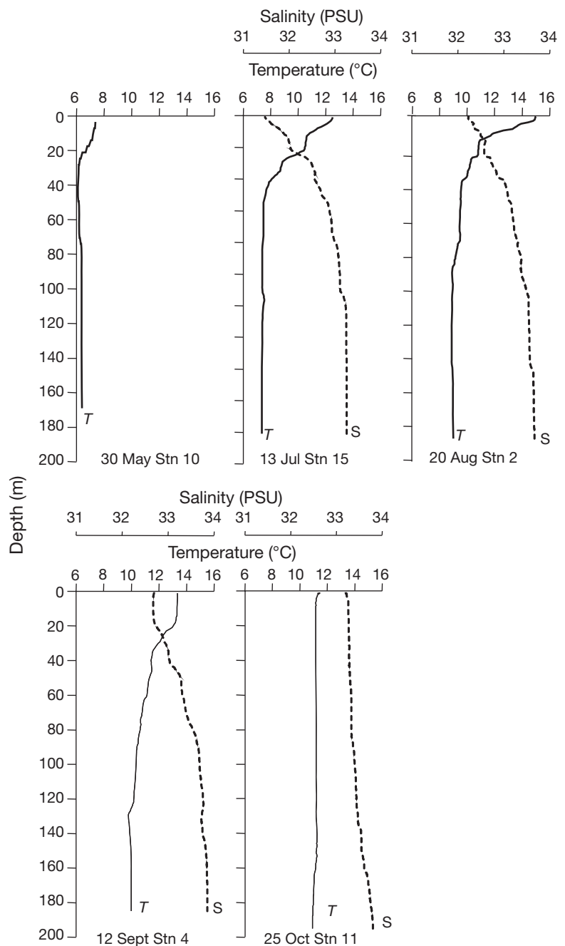
Fig. 2. Typical temperature ( T ; °C, solid) and salinity ( S , dashed) depth (m) profiles among several stations (see Fig. 1) and several days in the Grand Manan Basin associated with zooplankton sampling from May through October 2002. Temperature, salinity and thermocline depth ranges among all 46 stations over the sampling period are provided in Table 1
