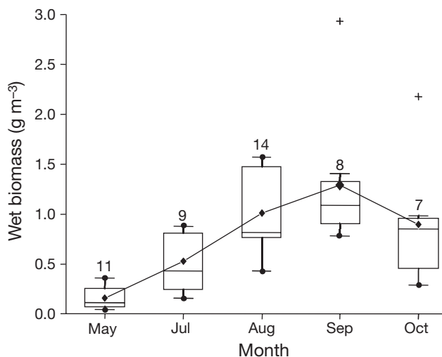
Fig. 3. Box and whisker summary of depth-integrated estimates of zooplankton wet biomass ( \text{g m}^{-3} ) in the Grand Manan Basin from May through October 2002. The box and line represent the lower quartile, median, and upper quartile, the diamonds represent the mean, and the whiskers represent 1.5× the inter-quartile range with outliers represented by crosses, absence of outliers by dots on the whisker. Numbers over box: no. of collections for each month
