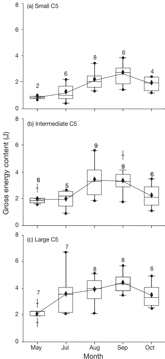
Fig. 6. Calanus finmarchicus . Box and whisker summary of depth-integrated estimates of: (a) small, (b) intermediate, and (c) large C. finmarchicus C5 individual gross energy content (EC, J) in the Grand Manan Basin from May through October 2002. The box and line represent the lower quartile, median, and upper quartile, the diamonds represent the mean and the whiskers represent 1.5× the inter-quartile range with outliers represented by crosses and absence of outliers by dots on the whisker. Numbers over box: no. of collections for each month
