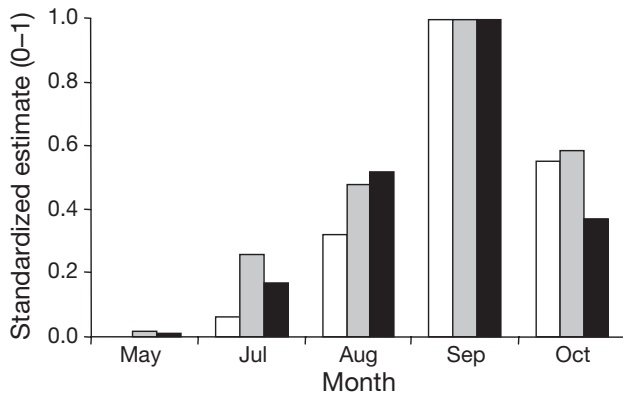
Fig. 12. Eubalaena glacialis and Calanus finmarchicus . Histograms illustrating parallel changes among the monthly standardized (0–1) estimates of right whale sightings per unit effort (whales \text{km}^{-1} survey track, open), depth-integrated concentration of C5s ( \text{m}^{-3} , shaded) and total energy density ( \text{kJ m}^{-3} , solid) in the Grand Manan Basin region during the period May through October 2002
