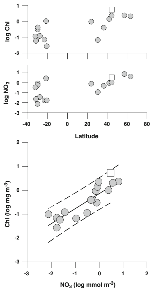
Fig. 8 Chlorophyll and nitrate concentrations in surface waters averaged into 16 biogeochemical ocean provinces indicating spatial distribution by latitude ( upper panels ) and the bivariate relationship, showing linear regression ( solid line ), 95% prediction limits ( dashed lines ), and long-term average state in Bedford Basin ( open square )
