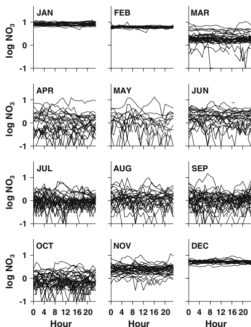
Fig. 2 Hourly records of nitrate ( \log \text{mmol m}^{-3} ) over the 24-h daily cycle from January 10 to December 31, 2007 in the Northwest Arm, displayed by month
