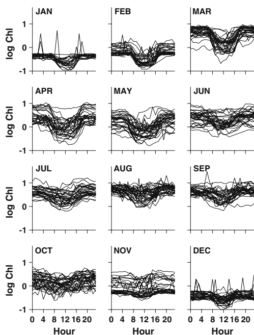
Fig. 1 Hourly records of in vivo fluorescence indicating chlorophyll ( \log \text{mg m}^{-3} ) over the 24-h daily cycle from January 10 to December 31, 2007 in the Northwest Arm, displayed by month
