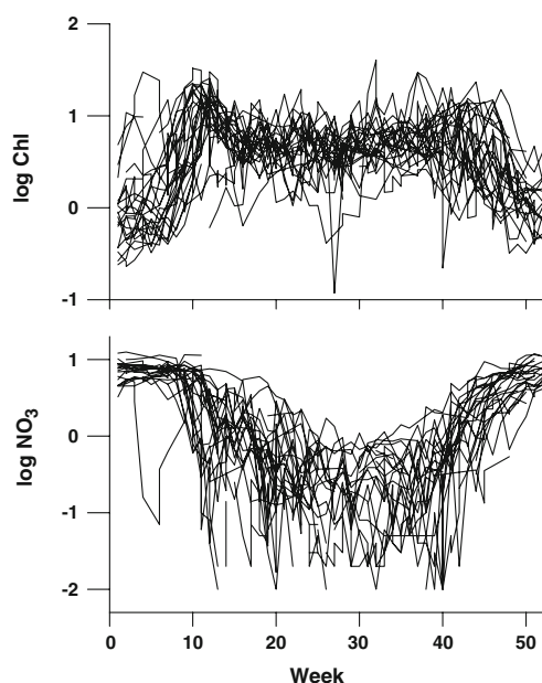
Fig. 3 Weekly records of chlorophyll ( \log \text{mg m}^{-3} ) and nitrate ( \log \text{mmol m}^{-3} ) over the 52-week annual cycle from 1967 to 2007 in the Bedford Basin
