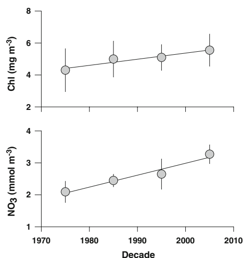
Fig. 6 Time series of chlorophyll ( \text{mg m}^{-3} ) and nitrate ( \text{mmol m}^{-3} ) averaged on a decadal basis. Error bars indicate intra-decade standard deviation
