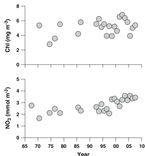
Fig. 4 Time series of chlorophyll ( \text{mg m}^{-3} ) and nitrate ( \text{mmol m}^{-3} ) averaged on an annual basis
