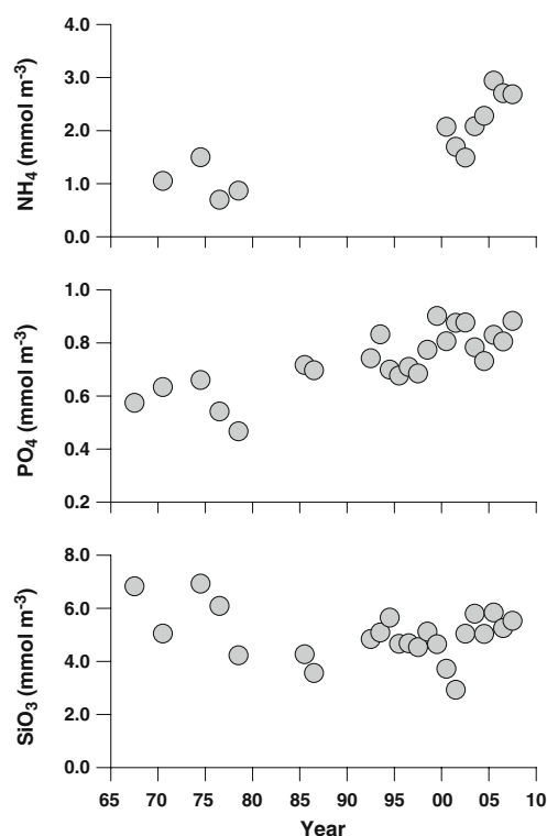
Fig. 5 Time series of ammonium ( \text{mmol m}^{-3} ), phosphate ( \text{mmol m}^{-3} ), and silicate ( \text{mmol m}^{-3} ) averaged on an annual basis
