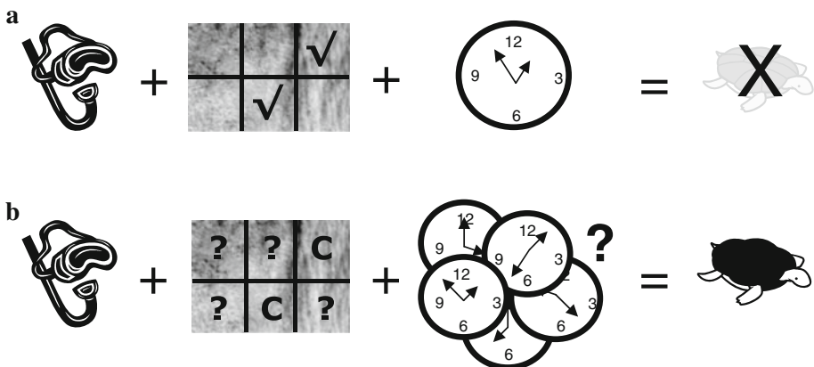
Fig. 1 Depiction of turtle avoidance behaviour where (a) illustrates daily tourist ( mask/snorkel ) occupation of zoned sea turtle habitat ( grid ) at the same location ( \checkmark ) and time ( clock ) that is expected to result in turtle avoidance behaviour ( x on turtle ) and (b) illustrates a temporally and spatially randomized turtle-watching schedule where the predicted result ( turtle = turtle viewing) accrues via the creation of ‘closed’ habitat areas ( c = habitat area closed to tours) and when other habitat locations and times are chosen randomly for turtle-watching tours (? = randomization of habitat location and time)
