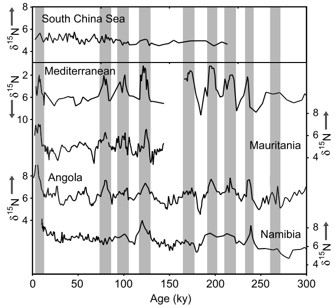
Figure 4. Sedimentary \delta^{15}\text{N} records from fixation, denitrification and well-mixed areas. Denitrification off W Africa is indicated by the \delta^{15}\text{N} records of Mauritania, Angola, and Namibia, as discussed in the text. The eastern Mediterranean [Calvert et al. , 1992] records low \delta^{15}\text{N} (note reversed axes), indicating nitrogen fixation, during the same periods as high denitrification is recorded on the African margin. Sedimentary \delta^{15}\text{N} records from the South China Sea [Kienast, 2000] are relatively invariant over the same time period, suggesting that this is a region of globally well-mixed N, which does not register changes in fixation or denitrification.
