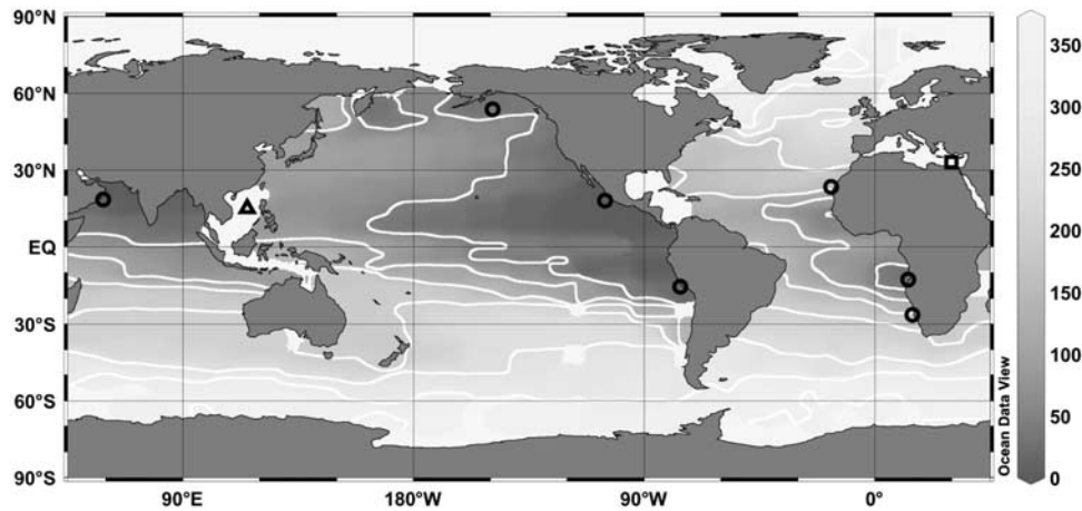
Figure 1. Dissolved O 2 (μmol/kg) on the 27.0 σ θ isopycnals; white contour lines are at 50 μmol/kg intervals. This potential density surface lies near the core of the AAIW and intersects the middepths of the world's WCD zones: the eastern tropical North Pacific, eastern tropical South Pacific, and Arabian Sea. Also visible are the low O 2 zones of Angola-Benguela, NW Africa, and the Subarctic Pacific. The locations of cores discussed in this paper are shown according to their dominant isotopic influence, as discussed in the text, indicated by a circle (denitrification), square (fixation), and triangle (mixed). Oxygen minima zones form where high oxidant demand, generated by the respiration of sinking organic matter from highly productive surface waters, coincides with low rates of oxygen renewal as determined by water mass circulation. Figure generated with Ocean Data View (R. Schlitzer, Ocean Data View, 2003; see http://www.awi-bremerhaven.de/GEO/ODV ) with the WOCE one-time data set.
