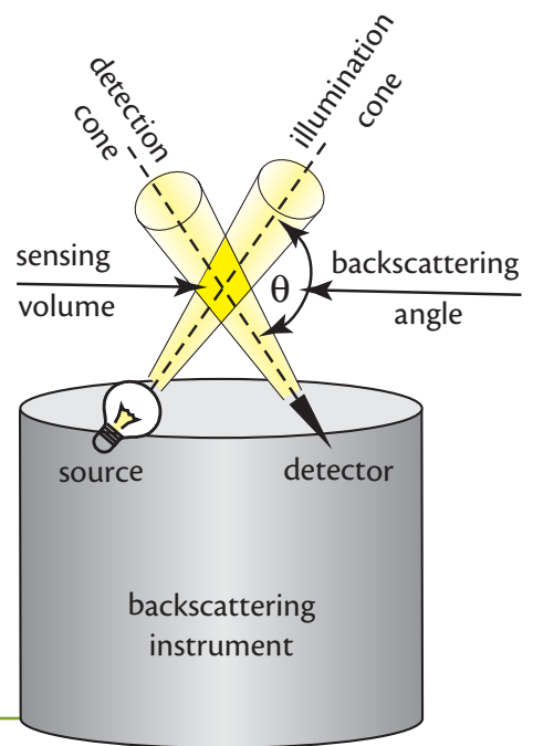
Figure 3. This schematic of a single-angle backscattering sensor shows a detector and source embedded within a flat-faced instrument. The light backscattered near the angle, \theta , emanates from the volume created by the intersection of the illumination and detection cones. The simple design of such sensors makes them ideal for deployment from small sensing platforms such as autonomous underwater vehicles and floats. The flat-face design can accommodate simple anti bio-fouling devices such as copper shutters.
