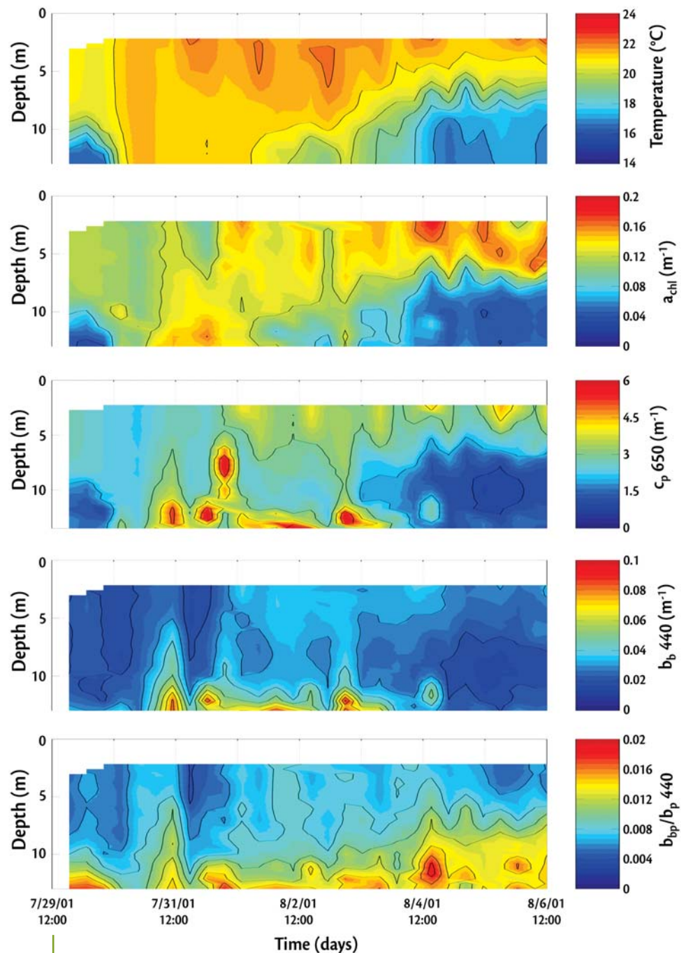
Figure 4. Eight-day time series of water temperature, chlorophyll absorption (based on the 676 nm absorption line height), beam attenuation coefficient at 650 nm ( c_{650} ), particulate backscattering coefficient at 440 nm ( b_{bp, 440} ), and the particulate backscattering ratio ( b_{bp}/b_p, 440 ; the ratio of particulate backscattering to particulate scattering) at 440 nm. All of these data were collected by the LEO-15 profiling mooring. Periods of a stratified water column (7/29 and 8/4-5/2001) are characterized by relatively low backscattering while a non-stratified period (7/30-8/3/2001) exhibit higher backscattering, in particular near the bottom due to sediment resuspension. The backscattering ratio is high near the bottom and low near the surface throughout the time series suggesting that high index of refraction sediments dominate near the bottom while low index of refraction phytoplankton dominate near the surface. This time series illustrates the added information that backscattering measurements provide to more traditional optical and hydrographical measurements.
